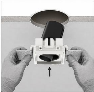
POSITION MESH WINGS / MARK FIXING POINTS
