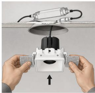
POSITION MESH WINGS / MARK FIXING POINTS
