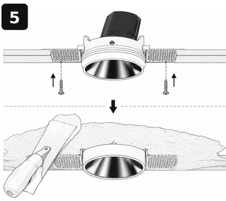
FIX MESH WINGS / APPLY PLASTER
