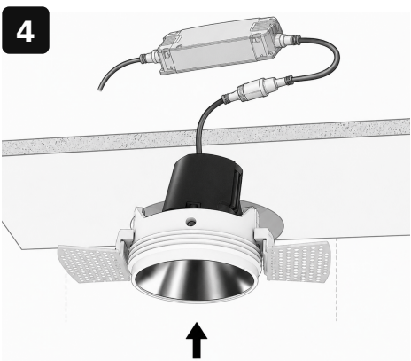
INSERT TRIMLESS HOUSING
