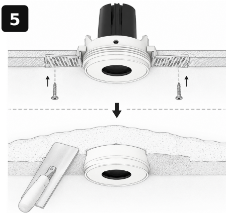
FIX MESH WINGS / APPLY PLASTER
