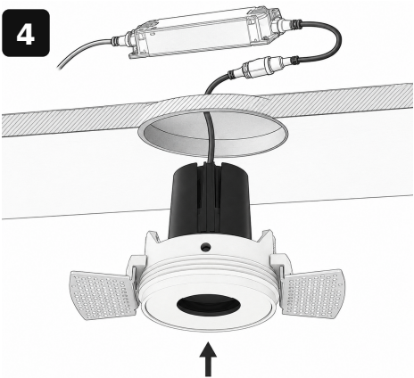
INSERT TRIMLESS HOUSING
